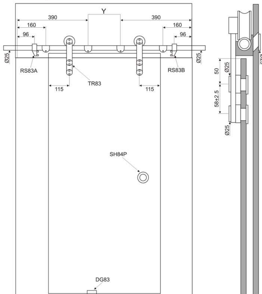
Roller Stopper RS83B
