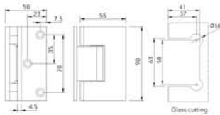
Glass cutting
