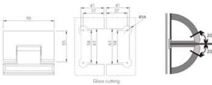
Glass cutting
