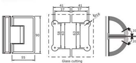
Glass cutting
