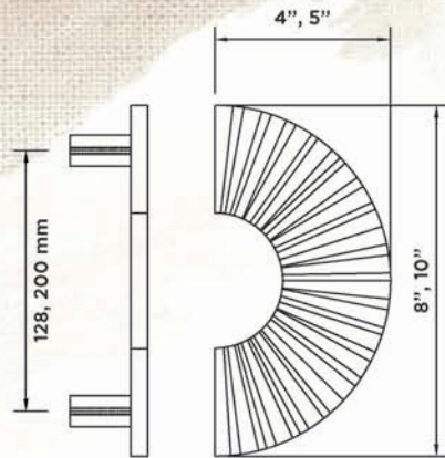
Sunshine Pull Handle
