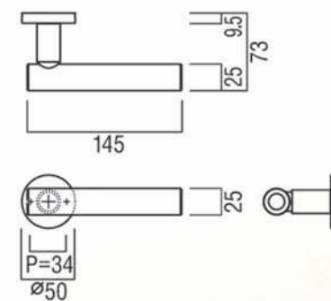
Lever Handle
