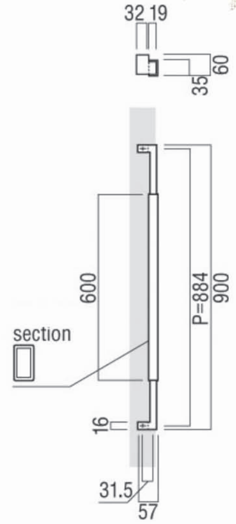
Fabio Pull Handle
