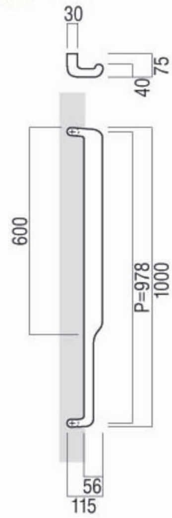
Xerxes Pull Handle
