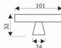
T Handle
