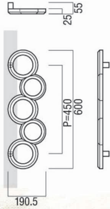
Oslo Pull Handle
