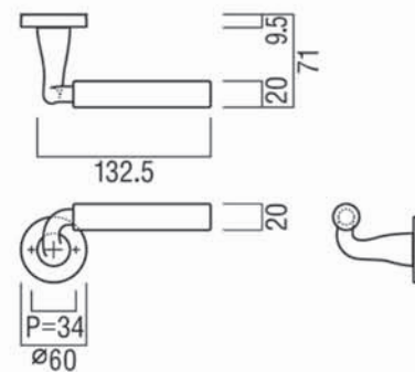
Lever Handle
