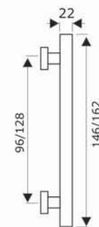
Cabinet Handle
