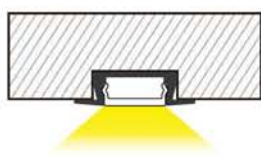
2. Recessed mounted or install with glue
