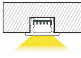
2. Recessed mounted, or install with glue
