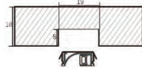
1. Slotting dimension 18mm width 8mm depth
