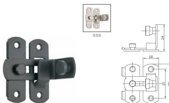
DCS207/S Sliding Security Lock
