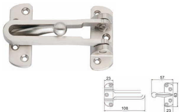
DGS200 - Stainless Steel Door Guard
