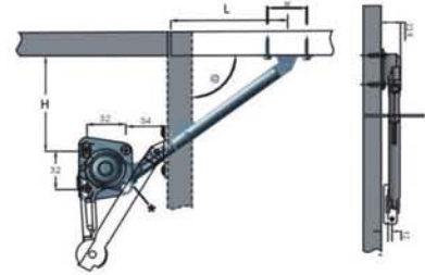
Installation illustration
