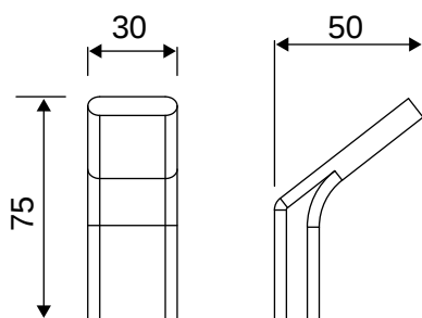
Hook BRH.501.CP
