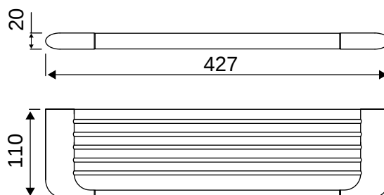
Shelf BSS.110.CP
